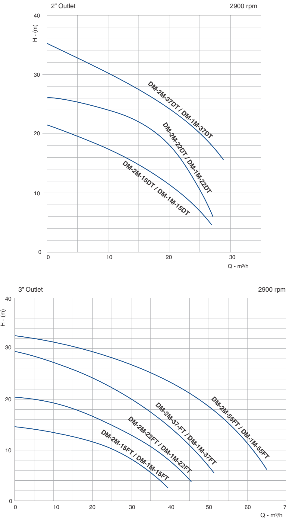
Performance Curves - DM Series
