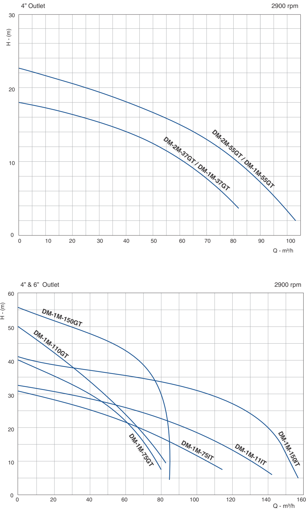
Performance Curves - DM Series
