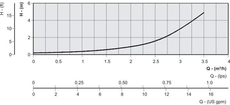
NPSH CURVE
